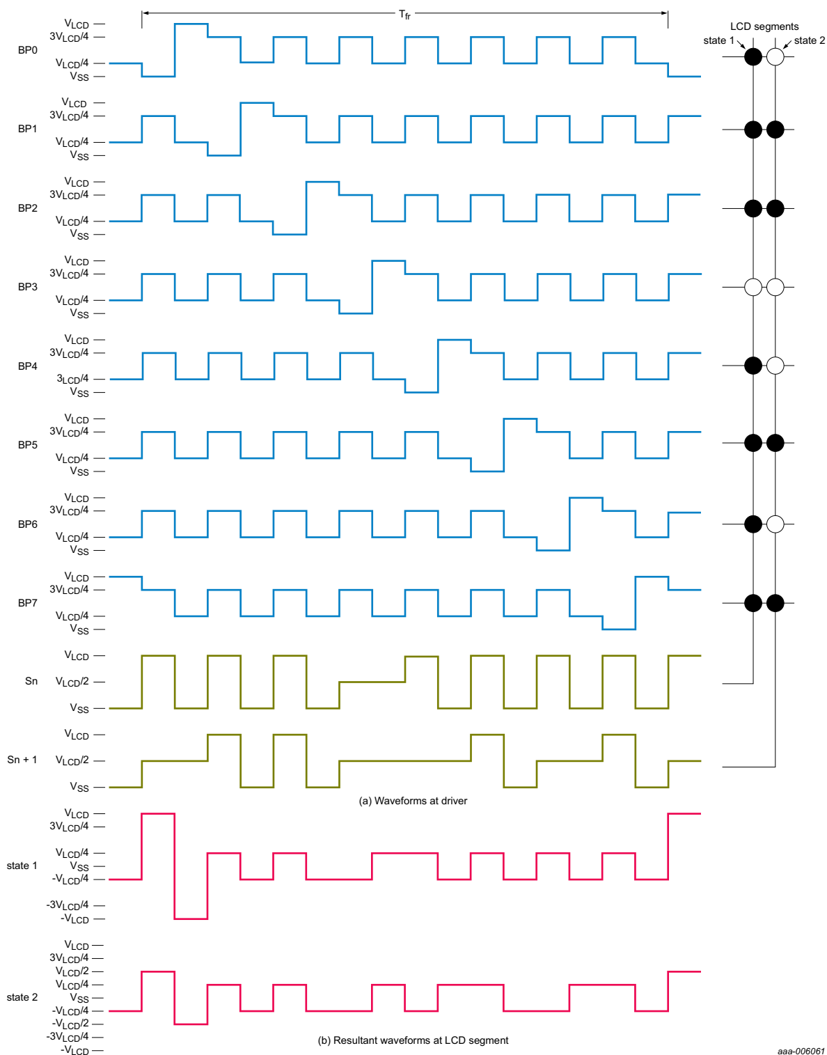
Fig 31. Waveforms for 1:8 multiplex drive mode, \frac{1}{4} bias, line inversion mode ( n = 1 )
